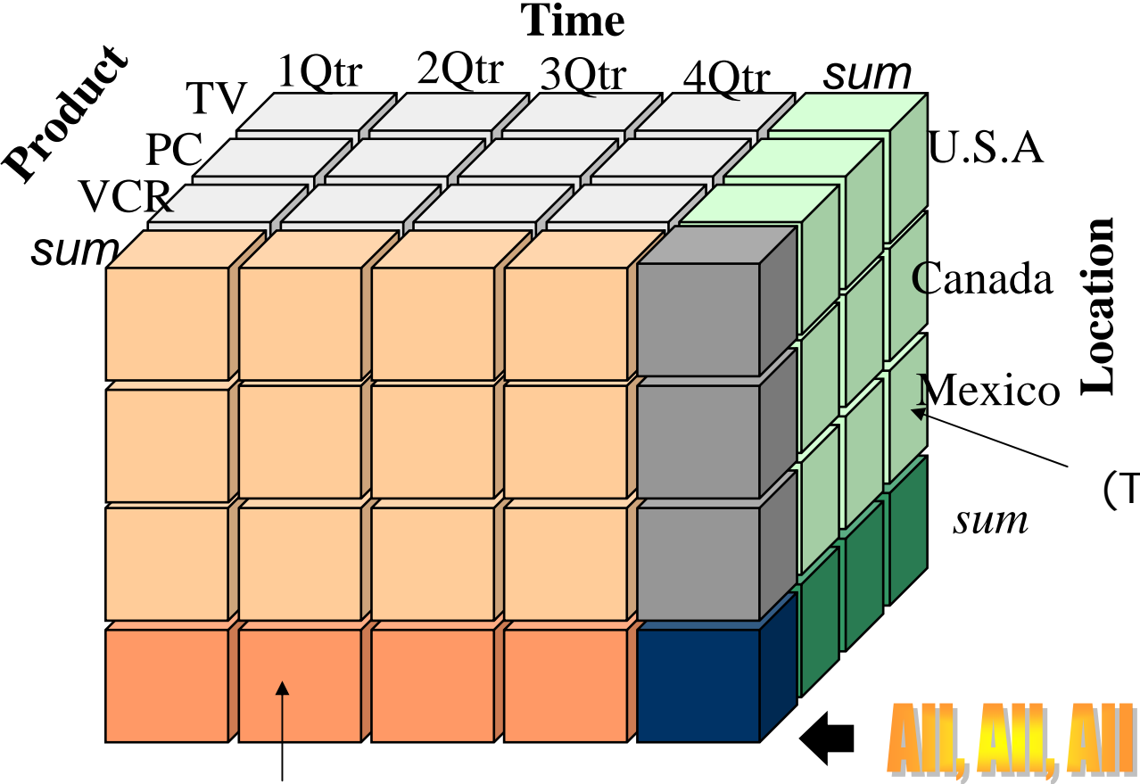
Derived cells, different levels of details
